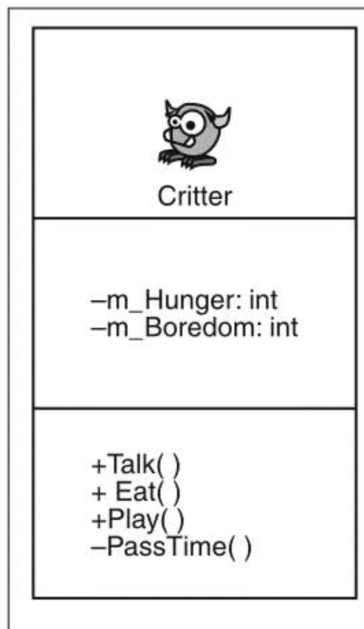
Figure 8.6 Model for the Critter class
