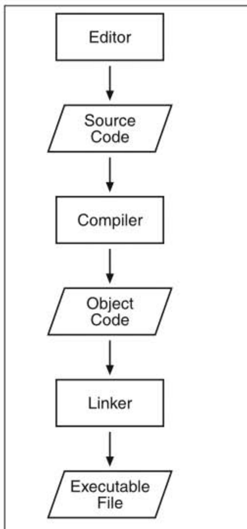
Figure 1.1 The creation of an executable file from C++ source code
